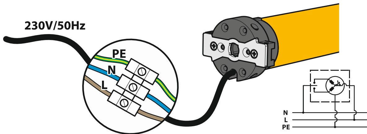
Fig.1 – Electrical interfaces
